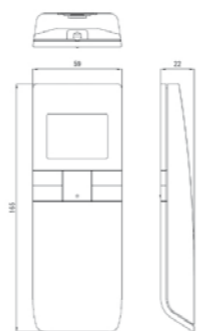
WIRELESS REMOTE CONTROLLER (CZ-RWS3)
